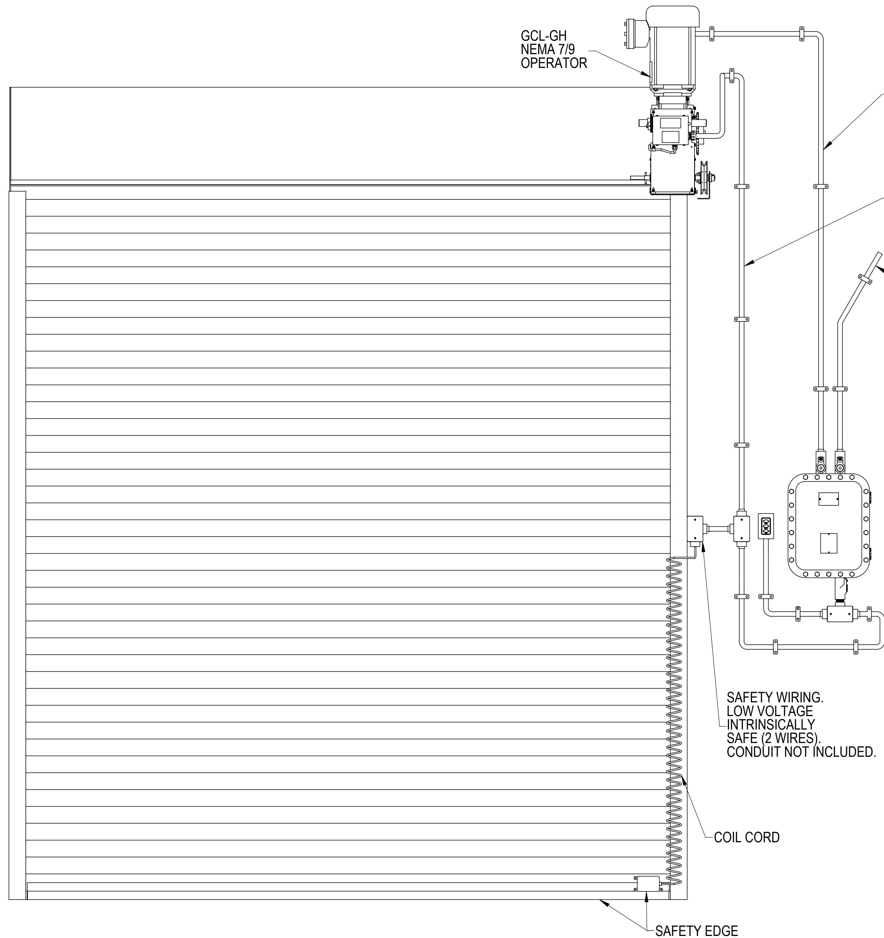
TYPICAL INSTALLATION
