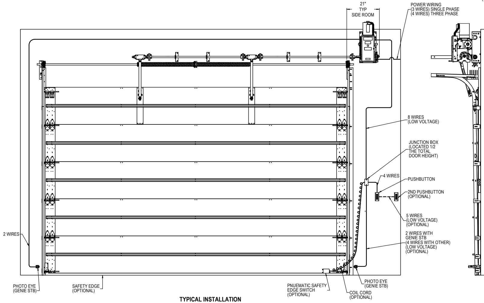
TYPICAL INSTALLATION
